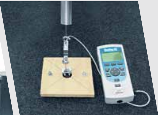
Testing of fixing element strength
