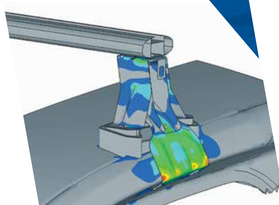
Simulation map of stress induced by roof rack tightening.
